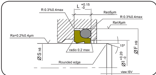
DOUBLE-LIP WIPER
