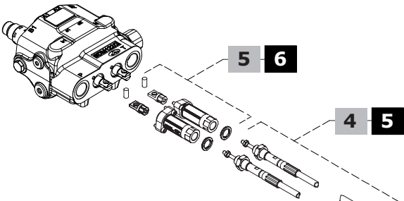
SDM122/2 directional control valve
